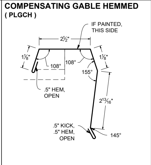
SCALE 1:3 S.O. 8.9375" WEIGHT: 7.9 LBS.
