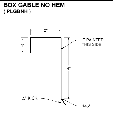
SCALE 1:3 S.O. 7.375" WEIGHT: 6.1 LBS.
