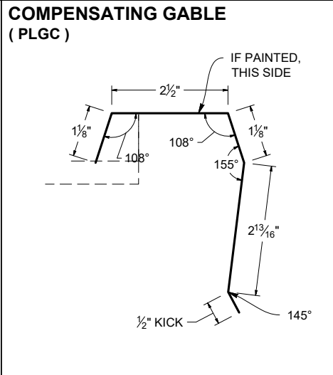
SCALE 1:3 S.O. 7.9375" WEIGHT: 6.6 LBS.
