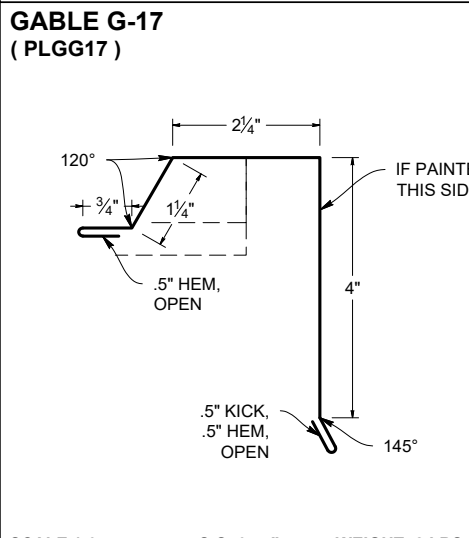
SCALE 1:3 S.O. 9.75" WEIGHT: 8 LBS.
