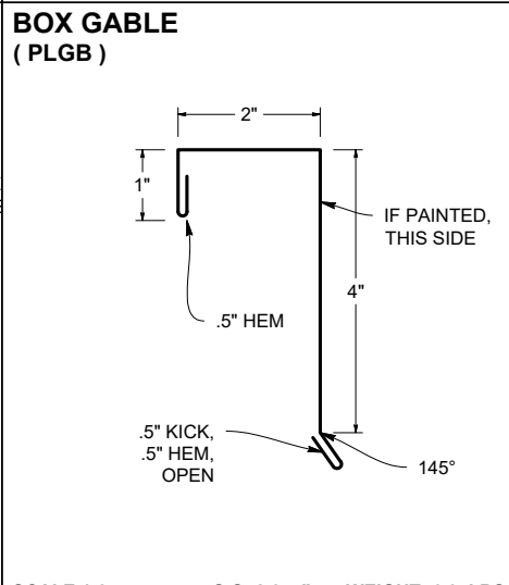
SCALE 1:3 S.O. 8.375" WEIGHT: 6.9 LBS.
