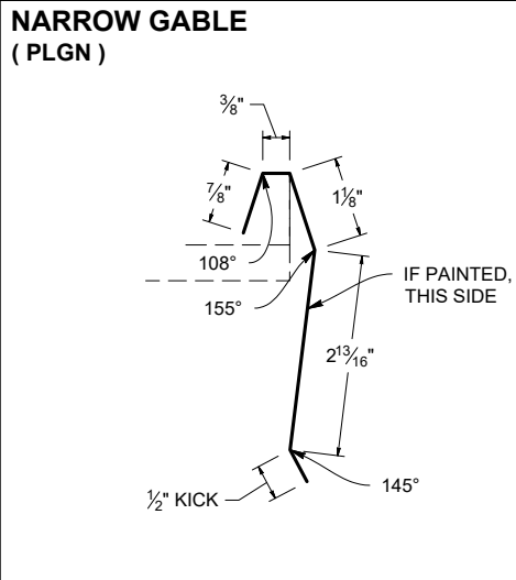
SCALE 1:3 S.O. 5.5625" WEIGHT: 4.7 LBS.
